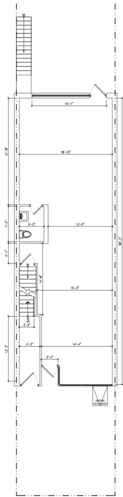
EXISTING 1ST PLAN
