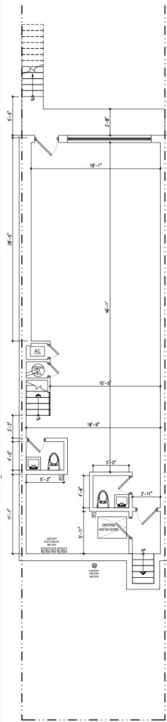
EXISTING CELLAR PLAN
