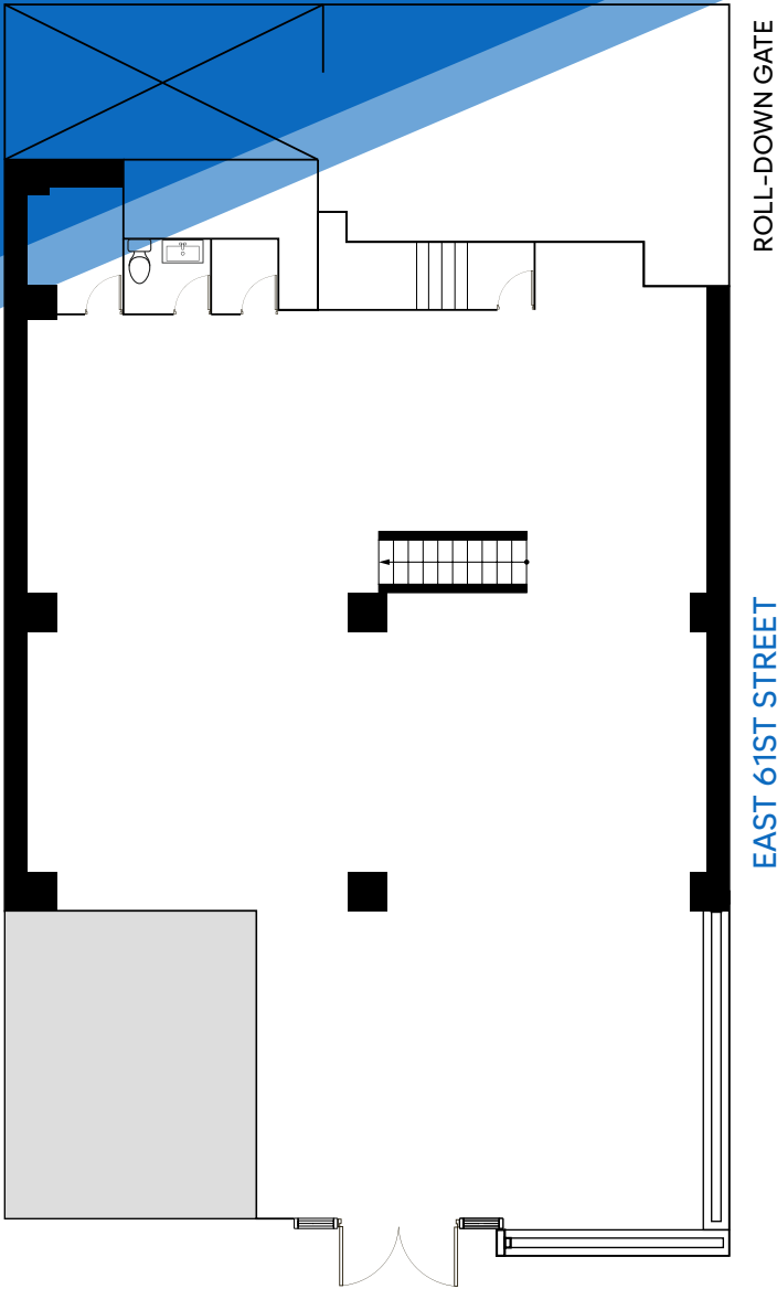
GROUND FLOOR
